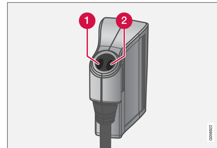
Charge module: 1. Red warning light, 2. Blue status indicator
