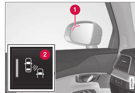
Location of BLIS indicator light. 76
