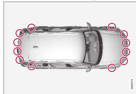
Parkeringssensorens placering 118 .
