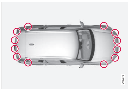
Parkeringssensorernas placering.
