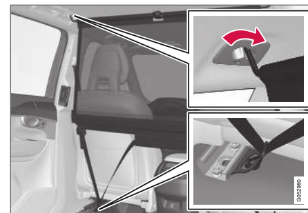
Främre montering.
