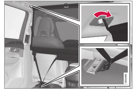
Montering foran.
