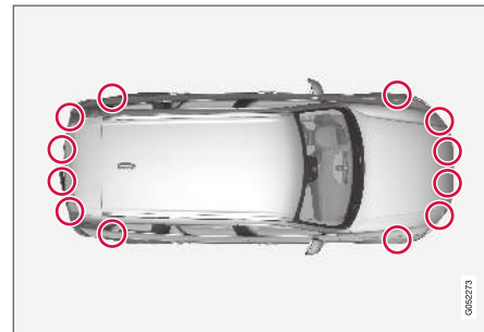
Parkeringssensorernes placering 125 .
