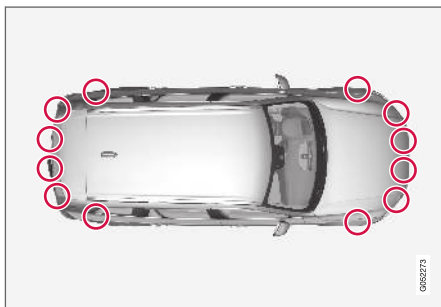
Parkeringsensorernes placering 139 .
