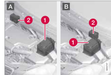
A: Left-hand drive car. B: Right-hand drive car. 1. Battery for starting 3 2. Support battery.
