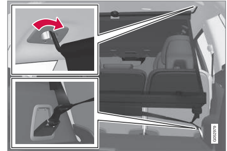
Rear mounting.
