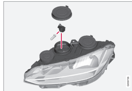
Venstre frontlys.
