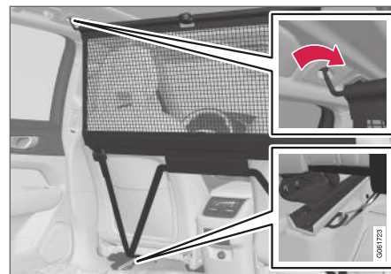
Främre montering.
